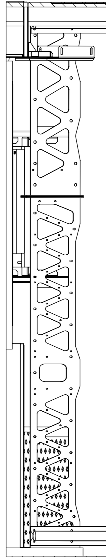
DETAIL C SCALE 1 : 10
